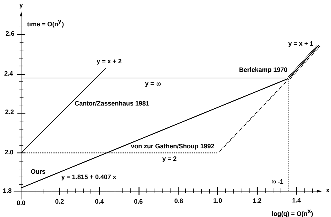
Figure 1: Running time comparisons for variable field cardinality
